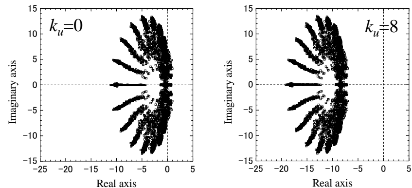
Variation of eigen value due to feedback
