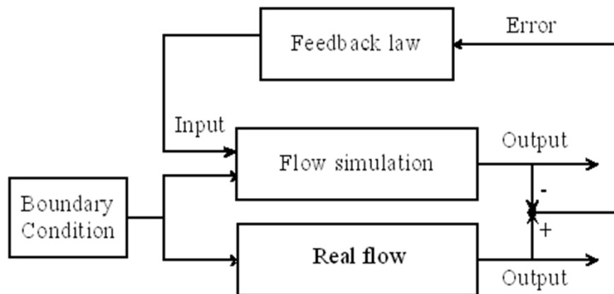
Block diagram of measurement-integrated simulation
