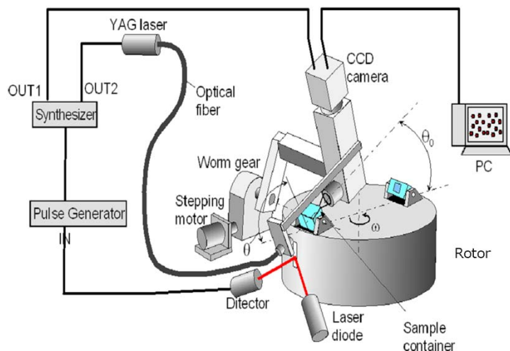
Inclined centrifuge microscope
