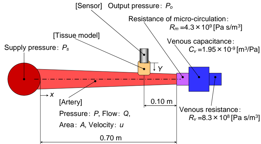
Numerical model of artery system in arm
