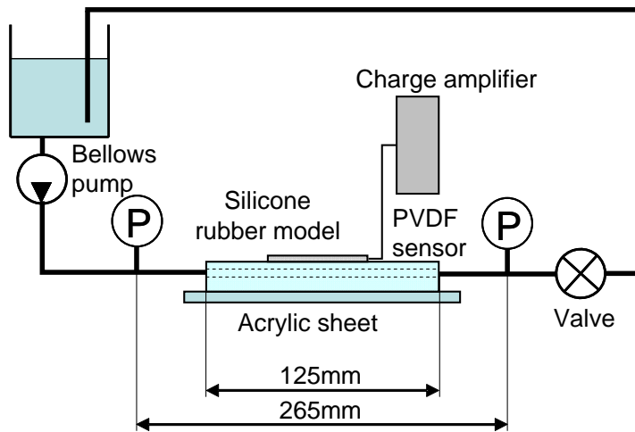
Experimental setup for pulse measurement with silicone model
