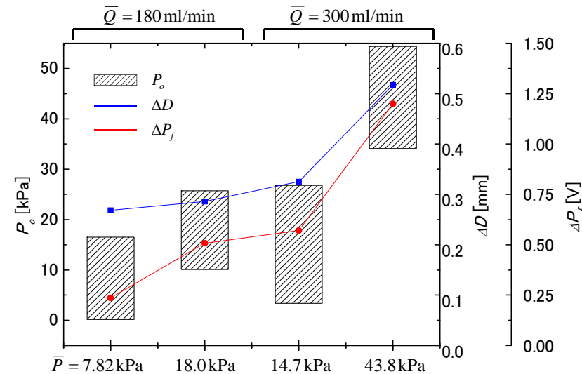
Variation of tube diameter and pulsation signal on various flow condition
